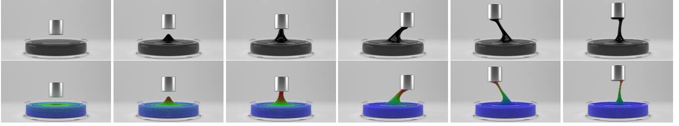
Fig. 4. A lump of magnetic viscous fluid in a container is attracted by a magnet, generating a spike.
